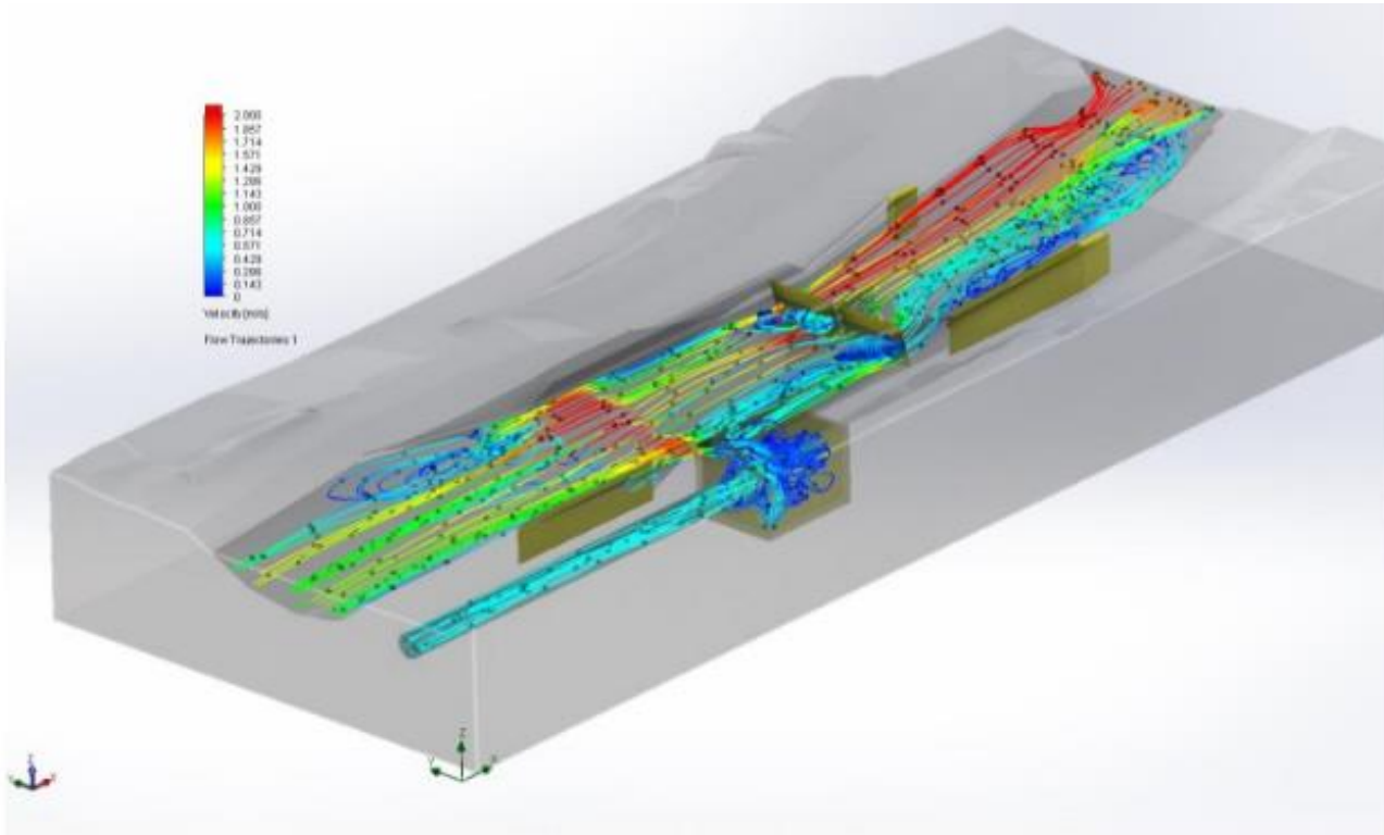
Figure A-6.1: Streamlines of New River flow during 1,200 cfs. flood conditions with 30% blockage of
